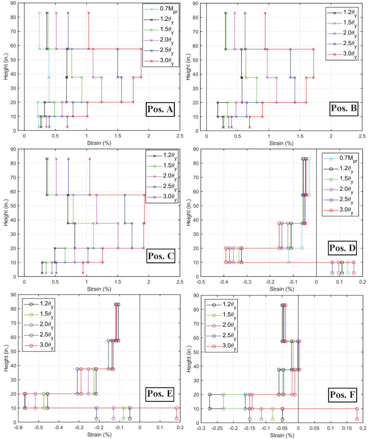
Figure 5-41: Axial strain profiles along the height of the edge of the East flange at different loading positions during the ramp-up loading of WLP, CW-2
