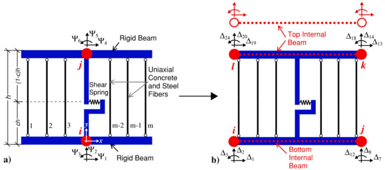
Figure 7-1: Transformation of a) 2-node MVLEM to b) 4-node MVLEM (Koložvari et al., 2021)
