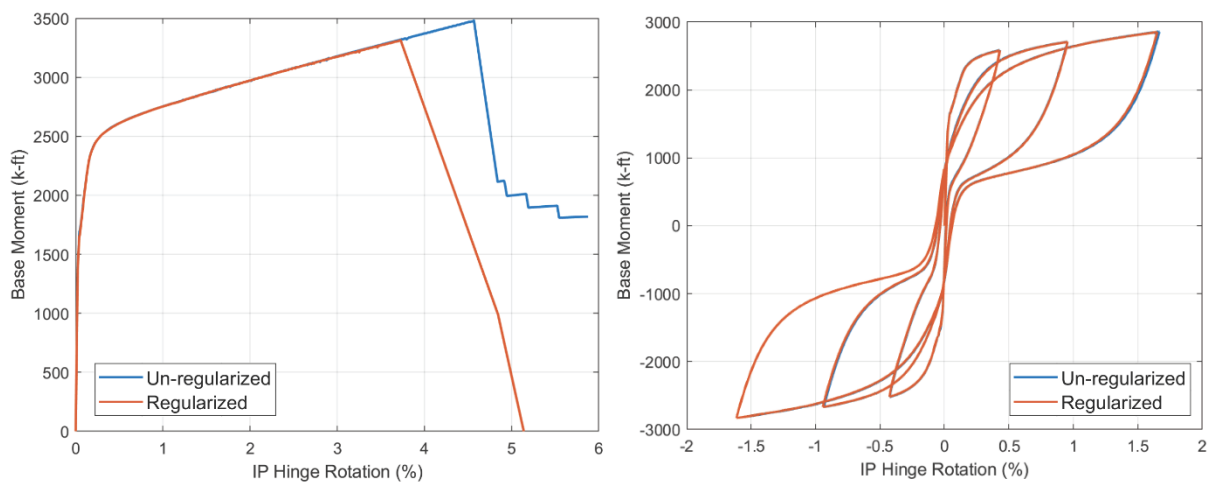
Figure 7-8: Effect of material regularization on monotonic (left) and cyclic (right) base moment-hinge rotation response of CW-1
