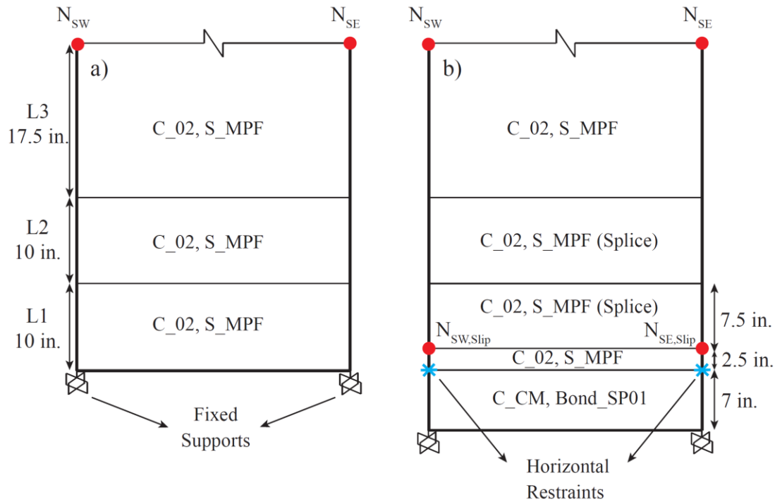
Figure 7-36: a) Original model and b) revised model with strain penetration elements
