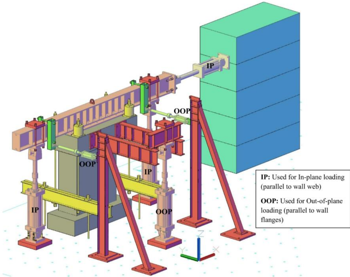
Figure 2-20: Isometric view of the test setup
