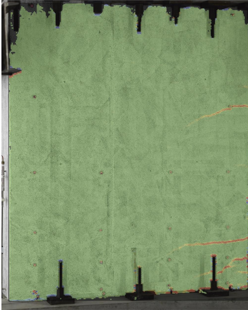
Figure 3-2: Crack pattern of the web obtained from DIC for CW-1 at the peak moment of the last cycle of 0.7M_{pr} moment demands under negative moment (Pos. A)
