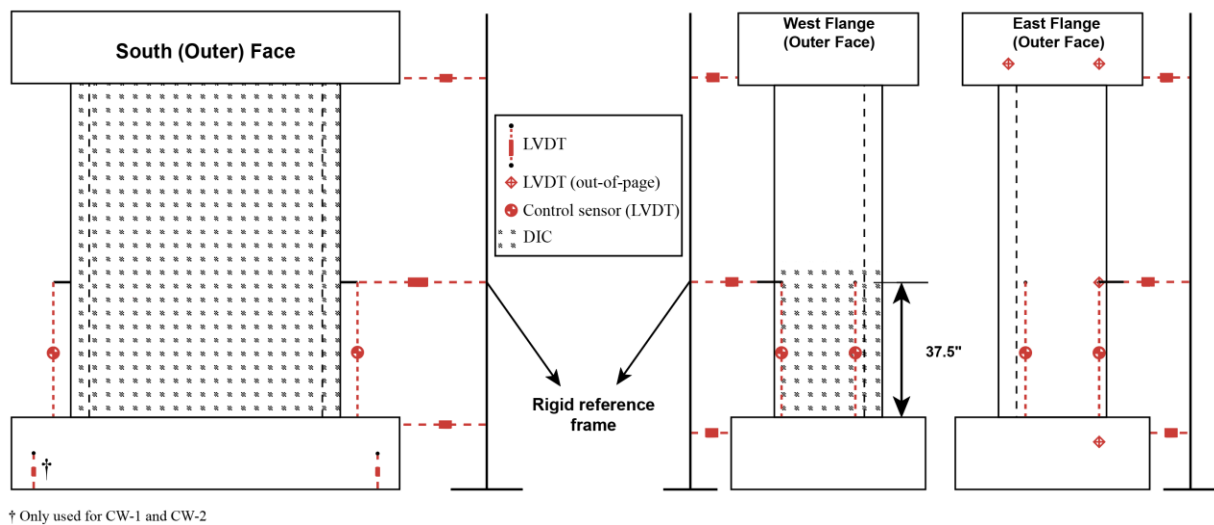
Figure 2-26: LVDT layout (control sensors and lateral displacements)
