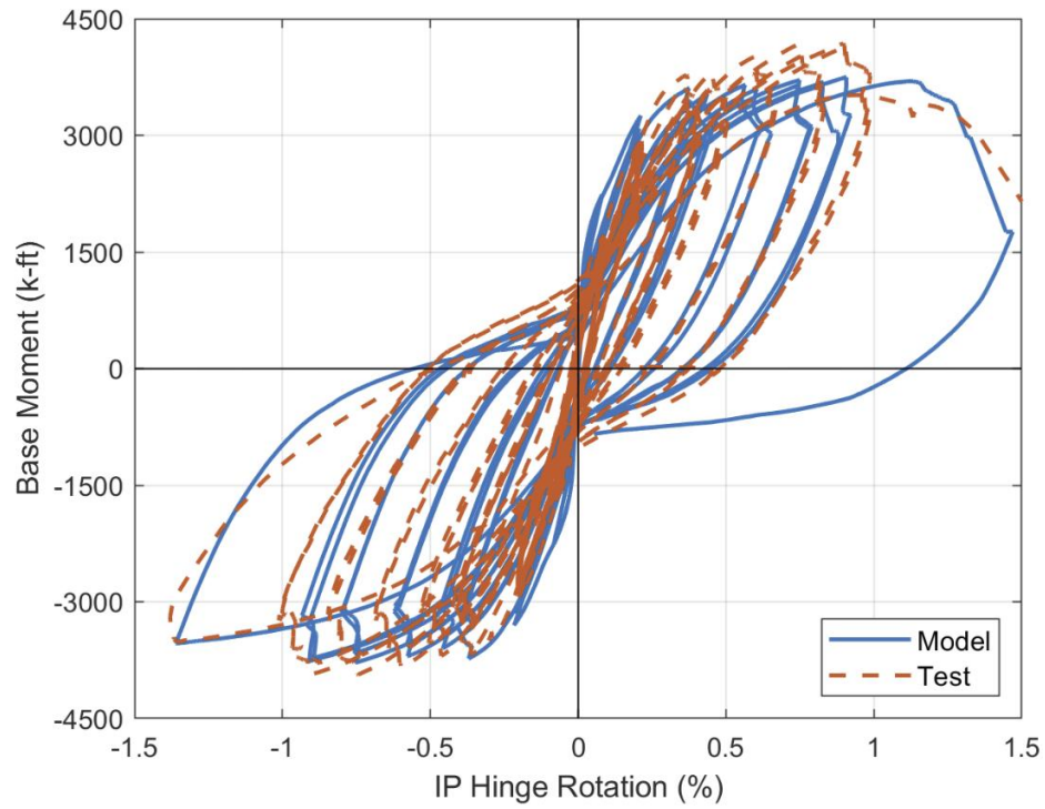
Figure 7-17: IP base moment-hinge rotation responses of CW-2
