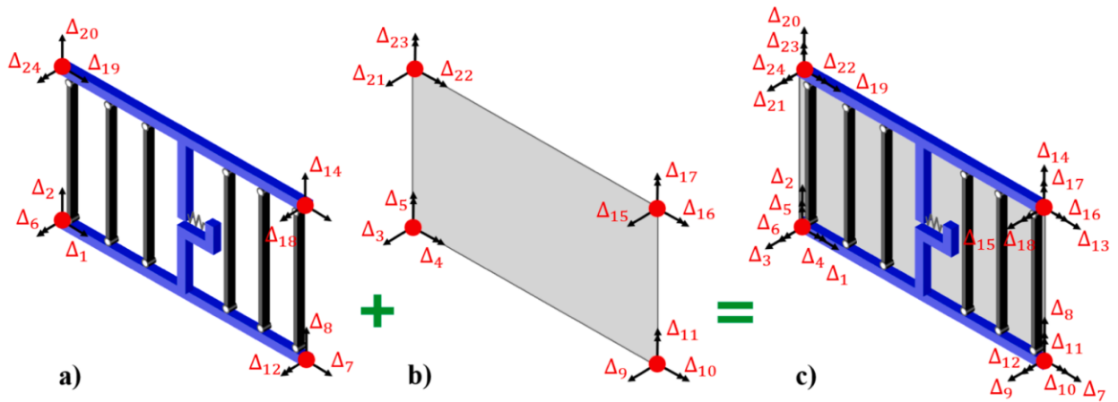
Figure 7-2: Formulation of MVLEM-3D (Koložvari et al., 2021)
