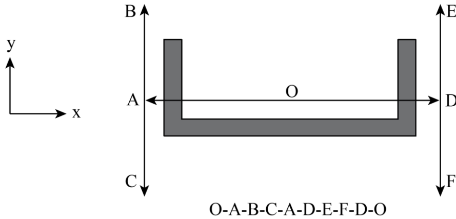
Figure 2-37: Biaxial loading scheme
