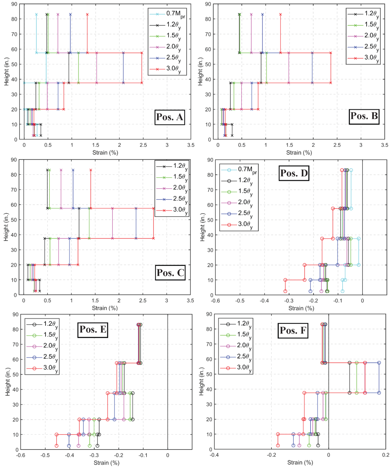
Figure 5-54: Axial strain profiles along the height of the edge of the East flange at different loading positions during the ramp-up loading of WLP, CW-4
