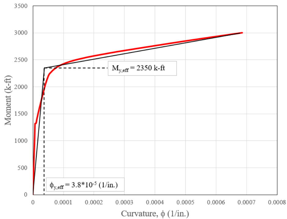
Figure F-3: Analytical moment-curvature response of CW-1 with effective yield moment and curvature values
