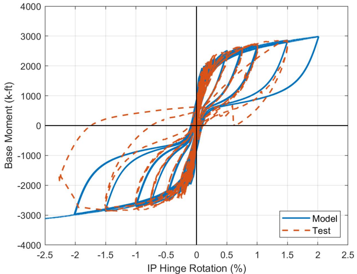
Figure 7-14: Base moment-hinge rotation responses of RCW-1
