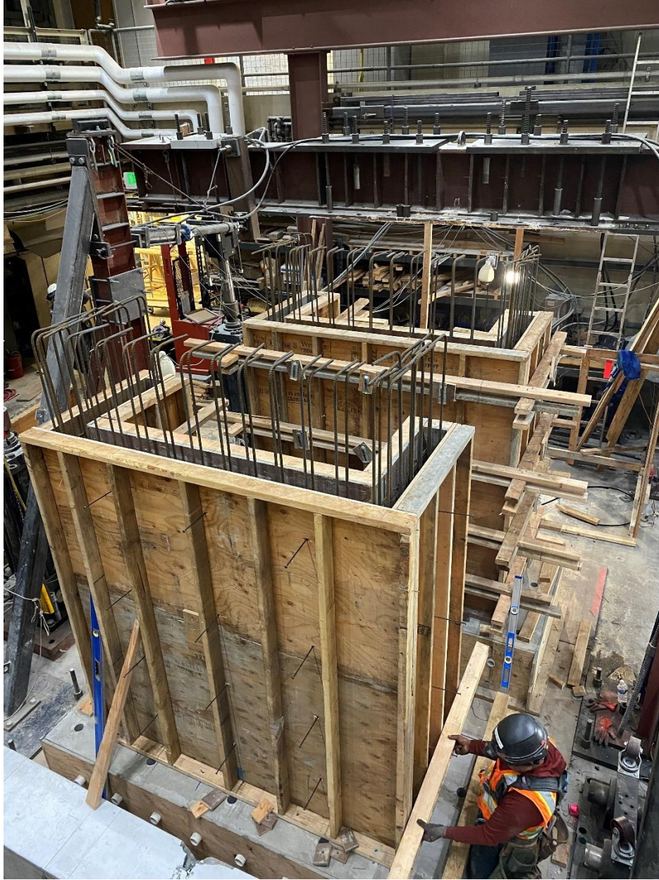
Figure D-12: Phase-II wall formwork
