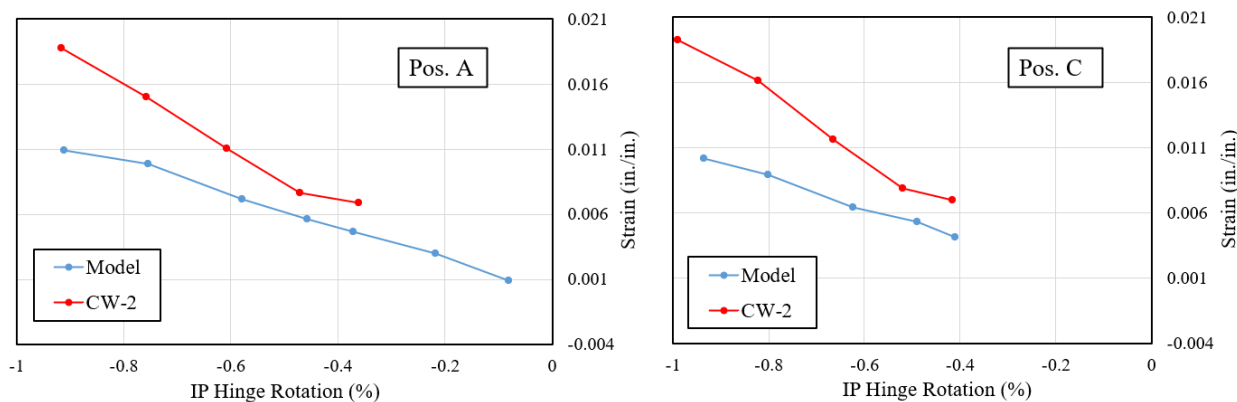
Figure 7-21: Comparison of tensile strains at the flange edges
