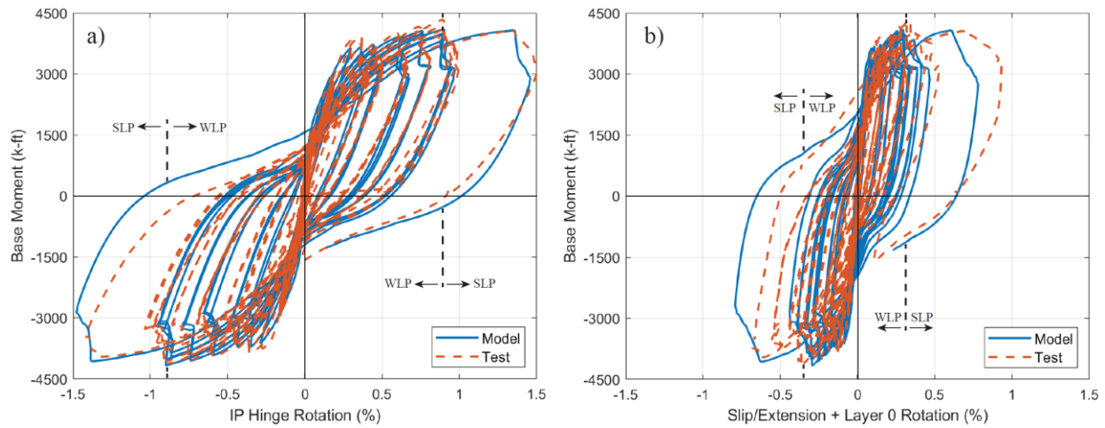
Figure 7-37: Advanced model results for CW-4, a) IP Base Moment – Hinge Rotation response and b) IP Base Moment – S/E Rotation response
