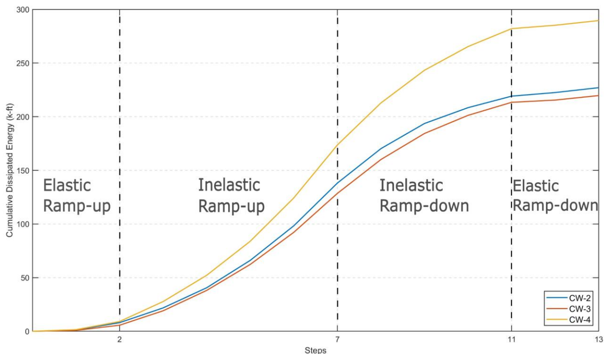
Figure 5-69: Total cumulative dissipated energy during WLP
