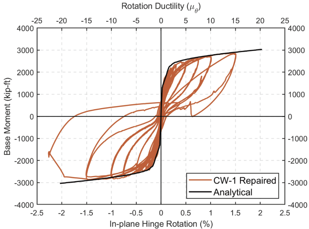
Figure 4-13: In-plane moment-hinge rotation response of RCW-1
