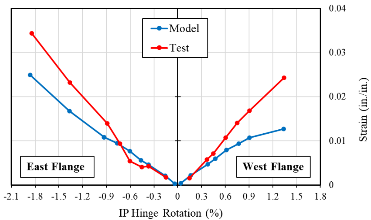
Figure 7-28: Comparison of tensile strains at the flange edges (Pos. A and D)
