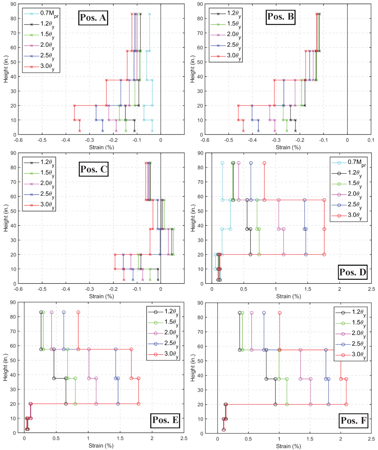
Figure 5-48: Axial strain profiles along the height of the edge of the West flange at different loading positions during the ramp-up loading of WLP, CW-3
