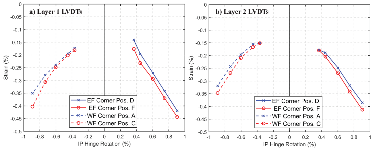
Figure 5-50: Comparison of compressive strains at different loading positions during the ramp-up loading of WLP for the first- and second-layer corner LVDTs, CW-3
