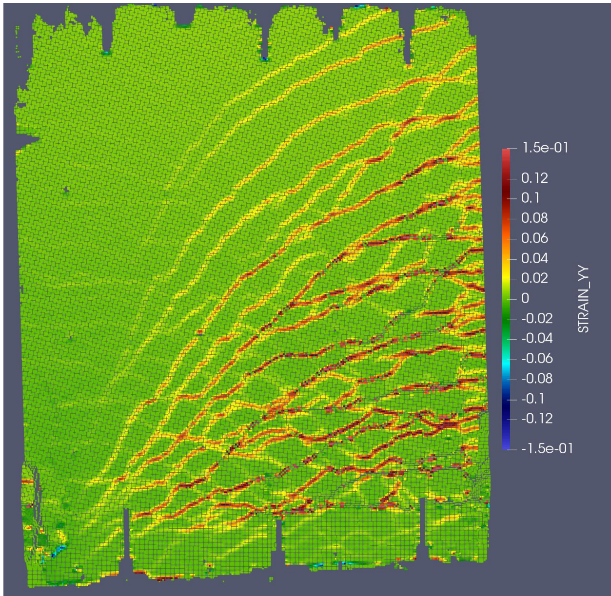
Figure 4-8: DIC analysis results at -2.0% rotation demands (first cycle)
