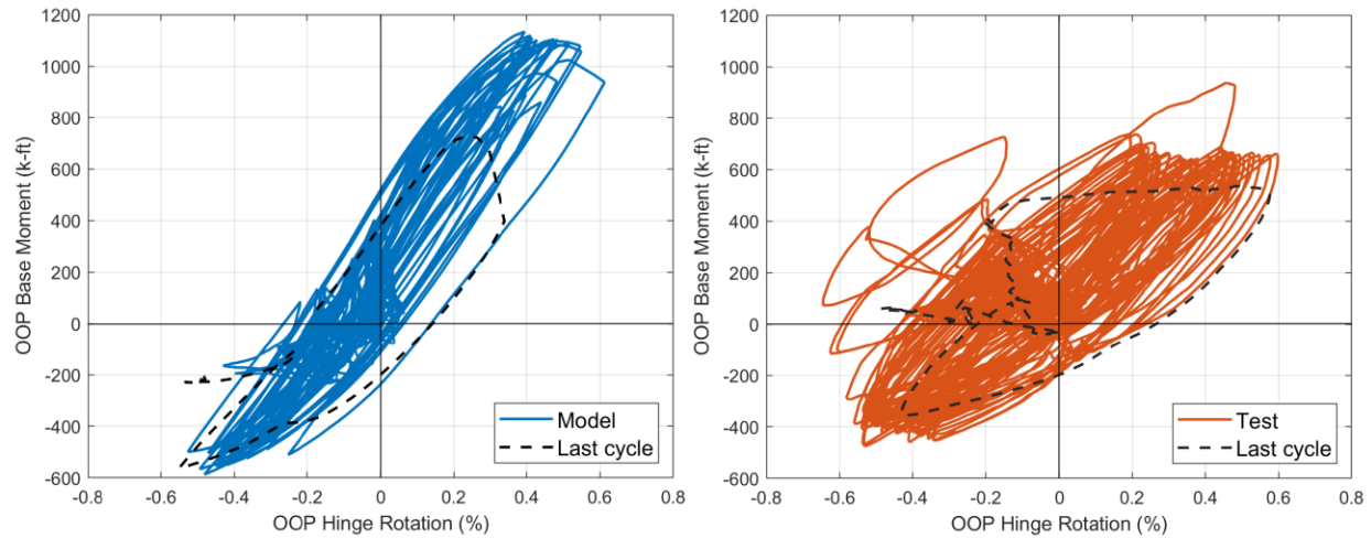
Figure 7-30: Comparison OOP base moment-hinge rotation responses
