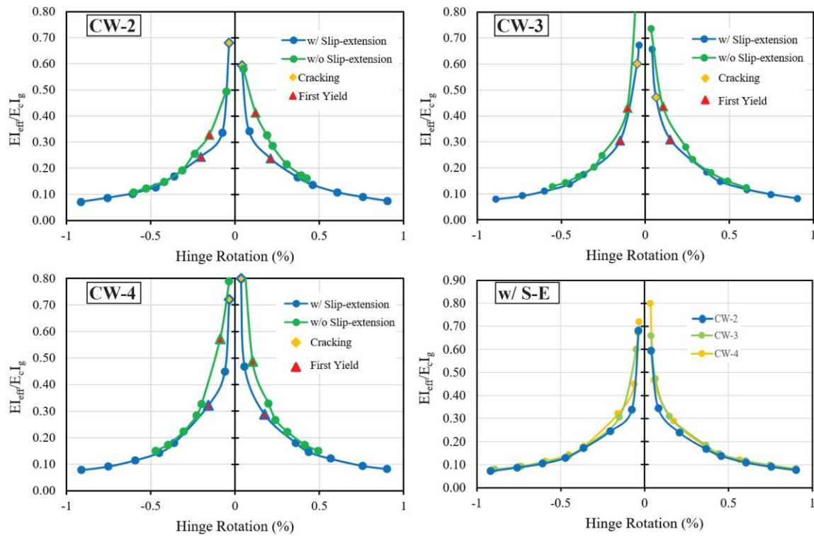
Figure 5-61: Normalized effective flexural stiffnesses ( EI_{eff}/E_cI_g )
