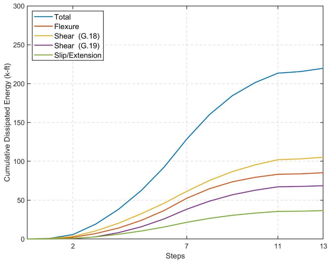
Figure 5-71: Cumulative dissipated energy due to different components of lateral displacement during WLP (CW-3)
