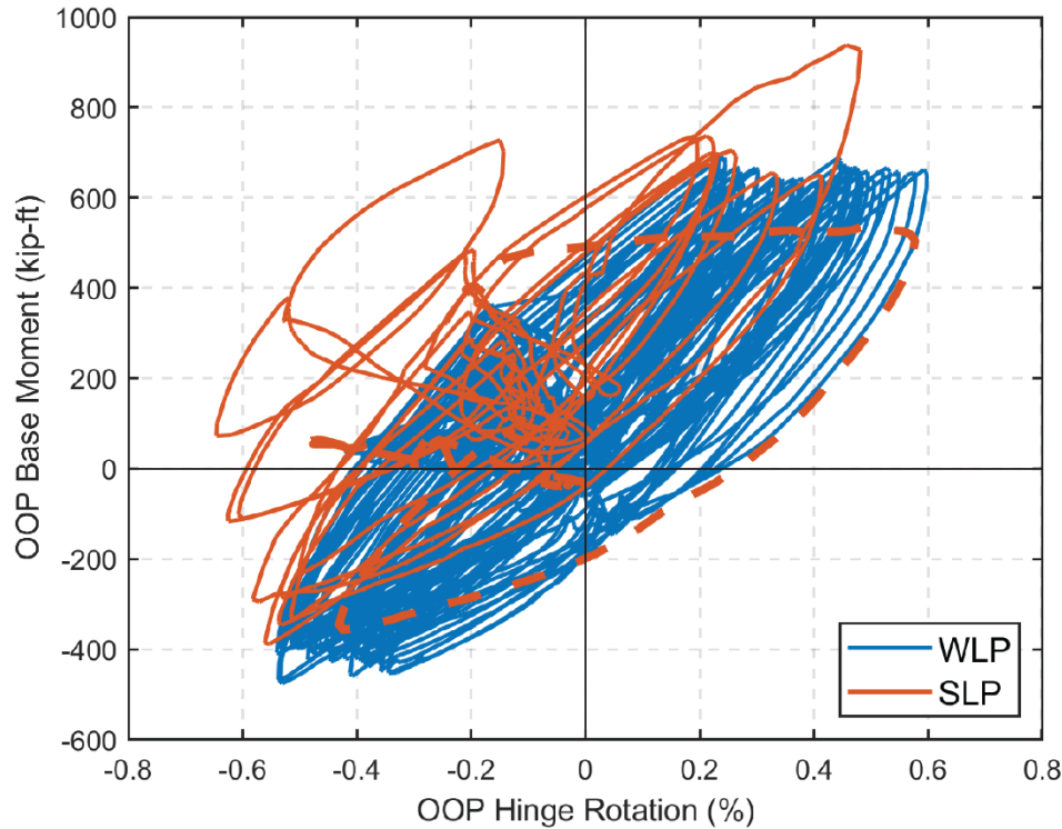
Figure 6-15: OOP Base moment-hinge rotation response of CW-4
