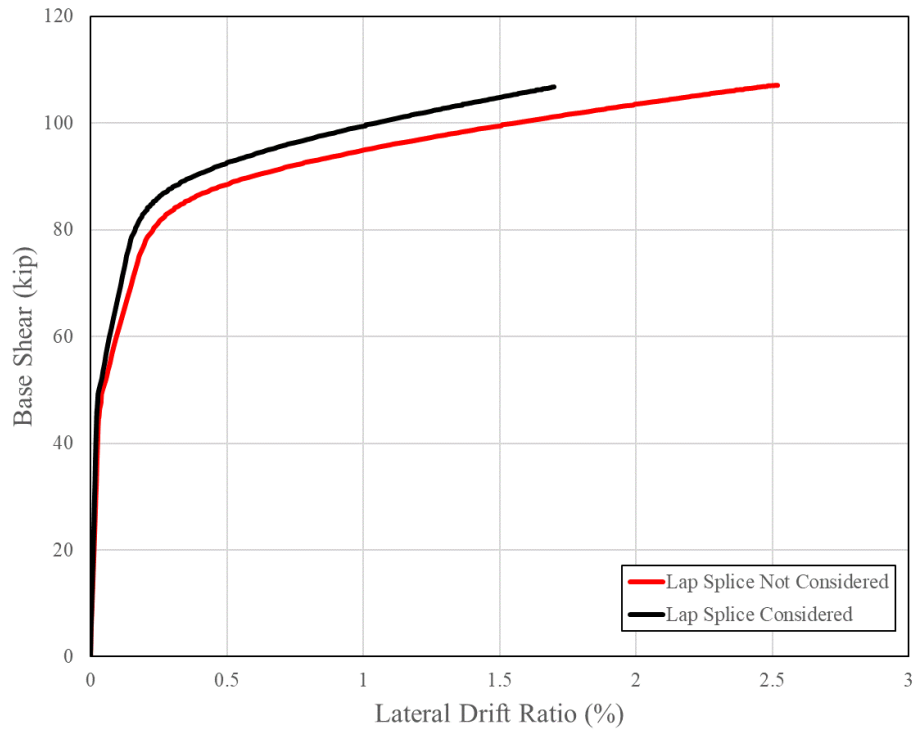
Figure G-4: Analytical shear-drift ratio response of CW-1
