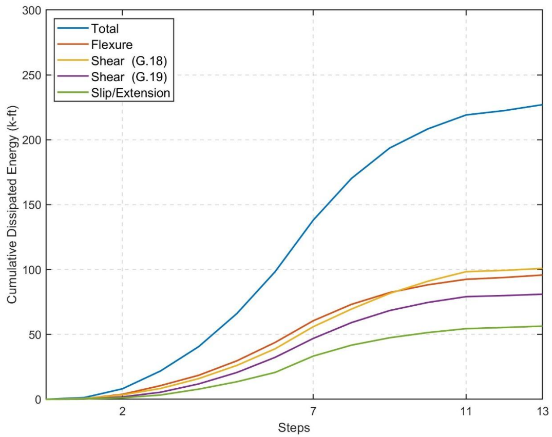
Figure 5-70: Cumulative dissipated energy due to different components of lateral displacement during WLP (CW-2)
