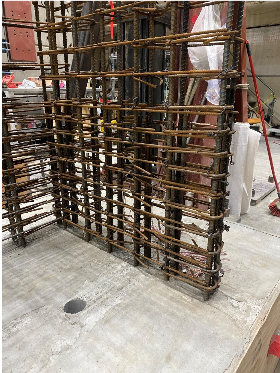
Figure D-11: CW-3 flange reinforcement close-up
