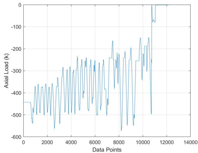
Figure 4-23: Axial load history of CW-1 during SLP
