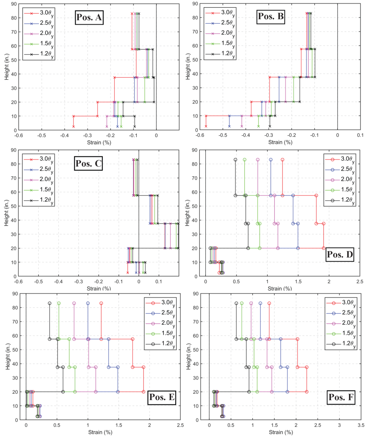
Figure H-6: Axial strain profiles along the height of the edge of the West flange at different loading positions during the ramp-down loading of WLP, CW-4
