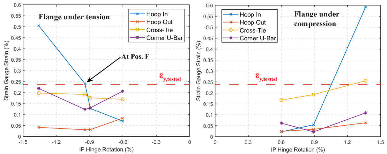
Figure 6-37: East flange transverse reinforcement strain gauge strains, CW-4
