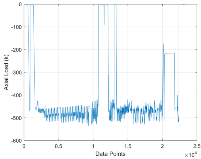
Figure 4-24: Axial load history of RCW-1
