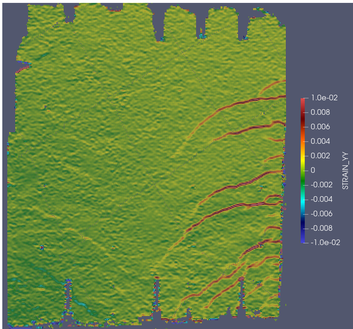
Figure 5-2: DIC analysis results at the last cycle of 0.4M pr demands at Pos. A, CW-2
