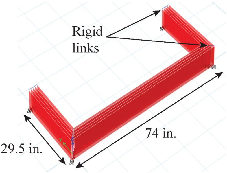
Figure 7-4: Five MVLEM-3D elements assigned to the flanges and the web (Detailed model)
