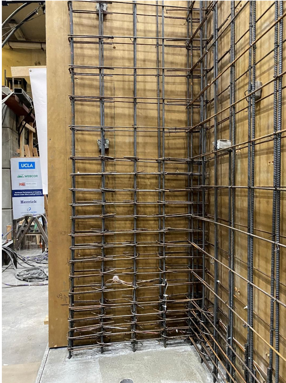
Figure D-4: CW-1 Flange reinforcement
