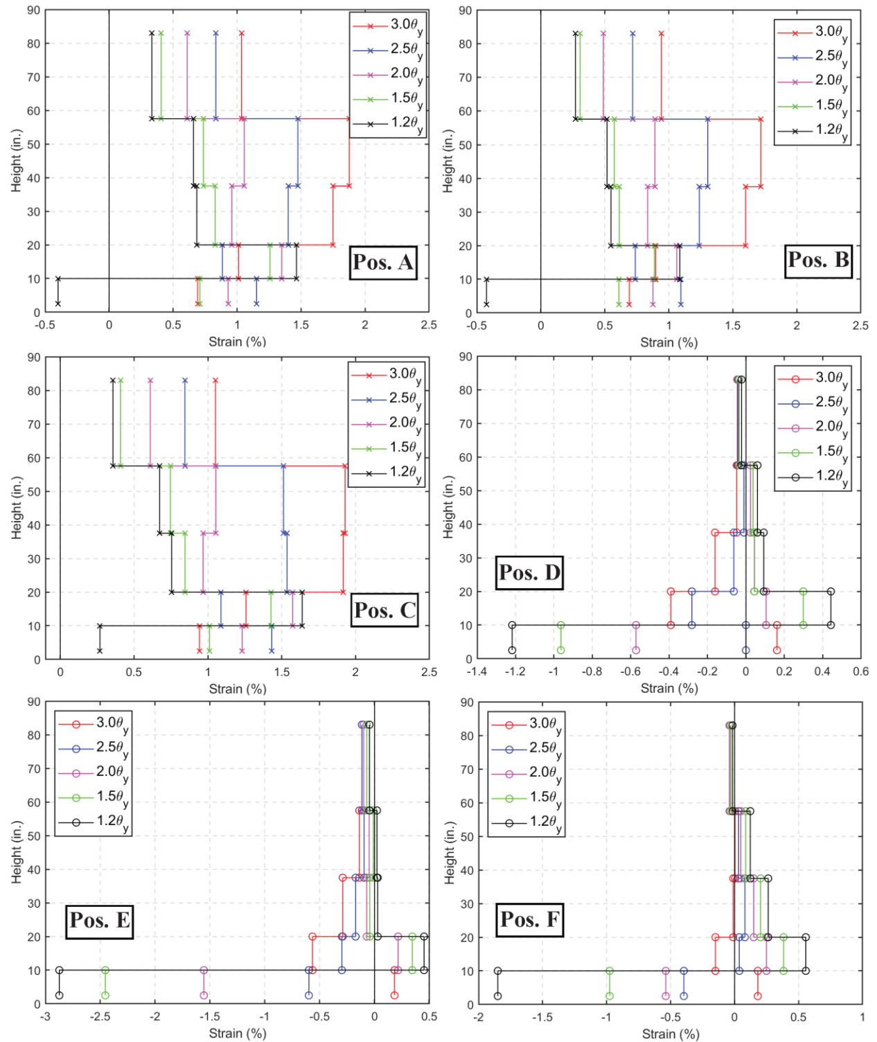
Figure H-1: Axial strain profiles along the height of the edge of the East flange at different loading positions during the ramp-down loading of WLP, CW-2
