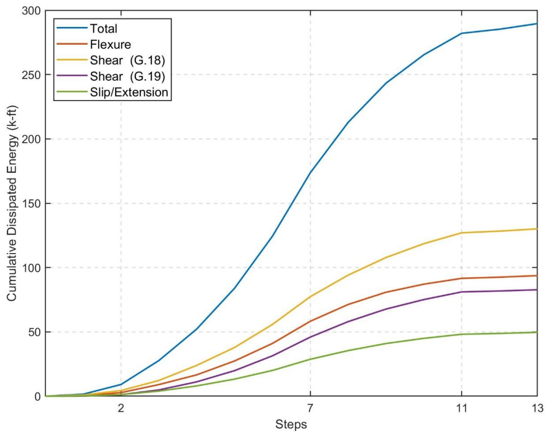
Figure 5-72: Cumulative dissipated energy due to different components of lateral displacement during WLP (CW-4)
