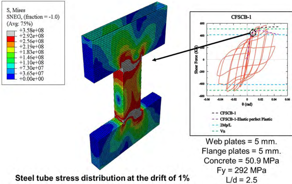
Figure 8-22. Comparison of monotonic response of finite element models with the experiment.
