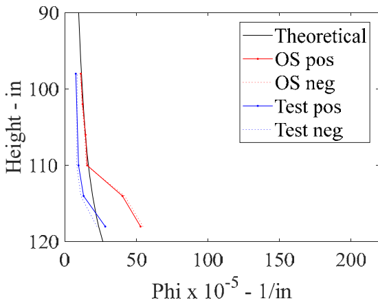
Figure 7-33. Moment curvature comparison for each linear potentiometer in Alzeni wall (Note that OpenSees results are on top of each other).
