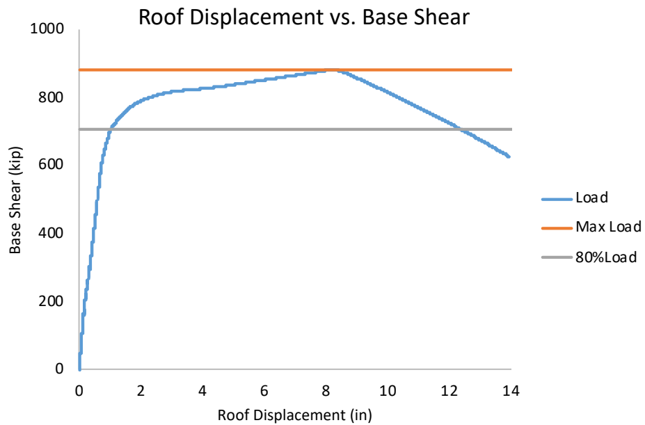
Figure 10-42. Base Shear versus Roof Displacement for Case 1.
