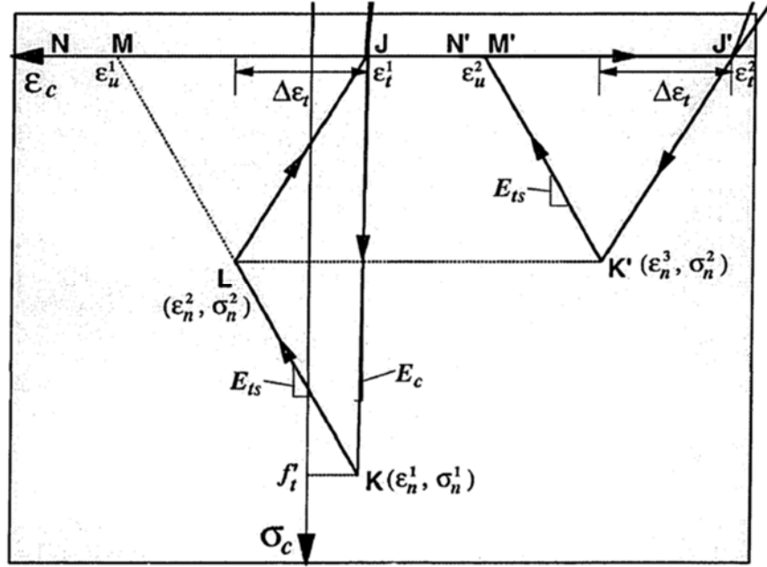
Figure A-18. Concrete model in tension (Hisham and Yassin 1994).
