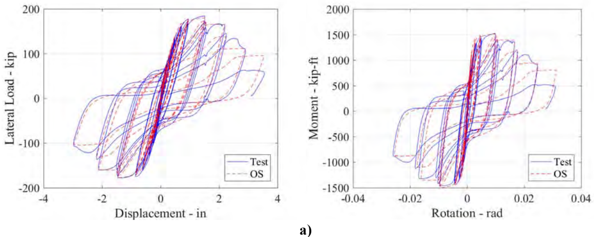
a) Figure 7-53. Base shear-displacement (left) and moment-rotation (right) comparisons of OpenSees models with test data for a) CW-42-55-10-T; b) CW-42-55-20-T; c) CW-42-14-20-T; d) CW-42-14-20-TS; and e) CW-42-55-30-T.
