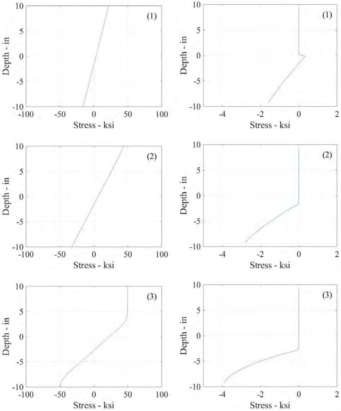
Figure 7-11. Stresses of a) steel; and b) concrete fracture-only cases in the composite cross-section
