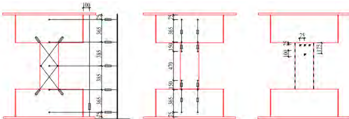
Figure 7-56. Instrumentation of coupling beams (dimensions are in mm.) (Nie et al. 2014).
