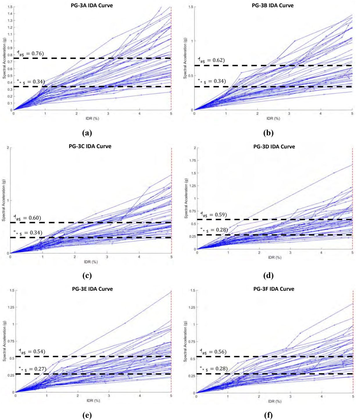
Figure 10-40. IDA curves for PG-3 structures – IMK with bilinear hinge (a) PG-3A 18-story D_{max} structure with L/d=3 , (b) PG-3B 18-story D_{max} structure with L/d=4 , (c) PG-3C 18-story D_{max} structure with L/d=5 , (d) PG-3D 22-story D_{max} structure with L/d=3 , (e) PG-3E 22-story D_{max} structure with L/d=4 , (f) PG-3F 22-story D_{max} structure with L/d=5 .
