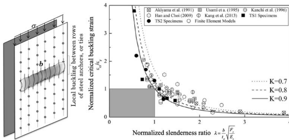
Figure 4-6. Local buckling of steel plates, and plot of normalized critical buckling strain vs. slenderness ratio (Zhang et al. 2014, 2019)
