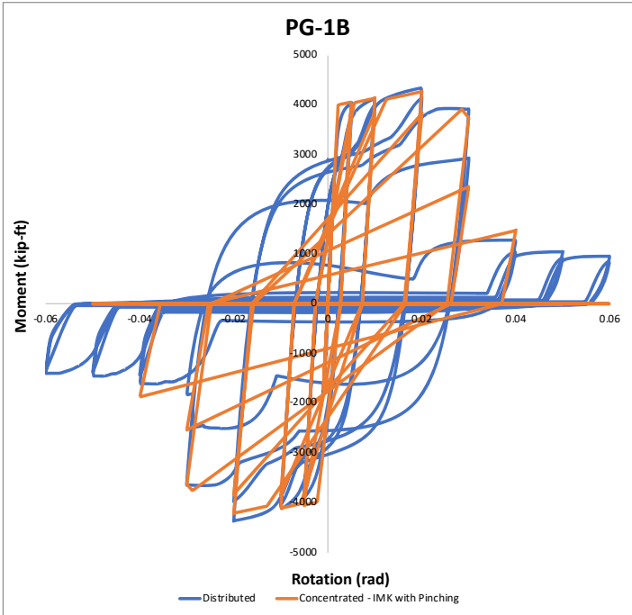
Figure 10-32. Moment versus rotation behavior for IMK with pinching hinge coupling beams of PG-1B.
