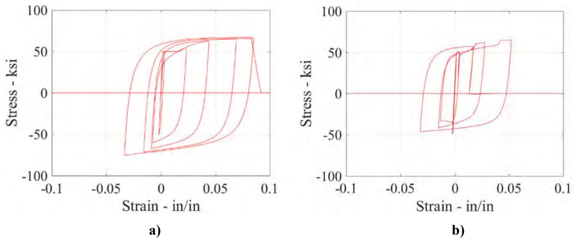
Figure 7-9. Stress-strain curve of outer most fiber in the composite section for a) fracture-only included and b) both fracture-and-buckling included cases
