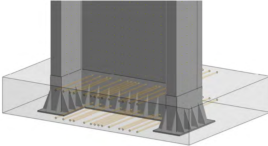
Figure 4-14. Composite wall-to-base connections with wall embedded into concrete foundation (Bruneau et al., 2019)
