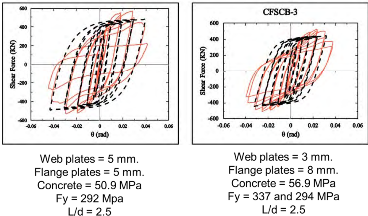
Figure 8-23.. Comparison of cyclic response of finite element models with the experiment.
