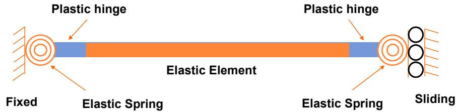
Figure 8-36. Graphical representation of coupling beam distributed plasticity model.
