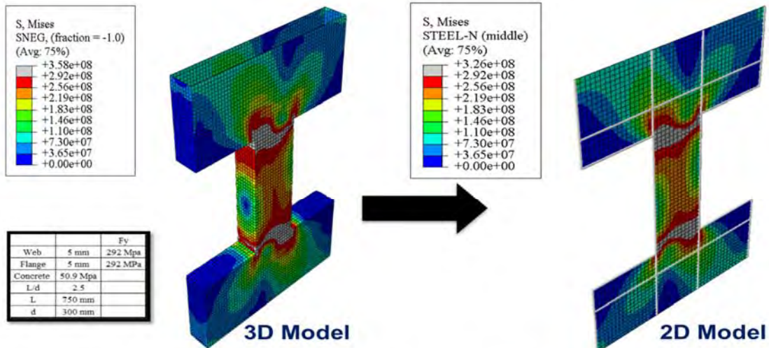
The von Mises stress distribution at the drift of 1%
