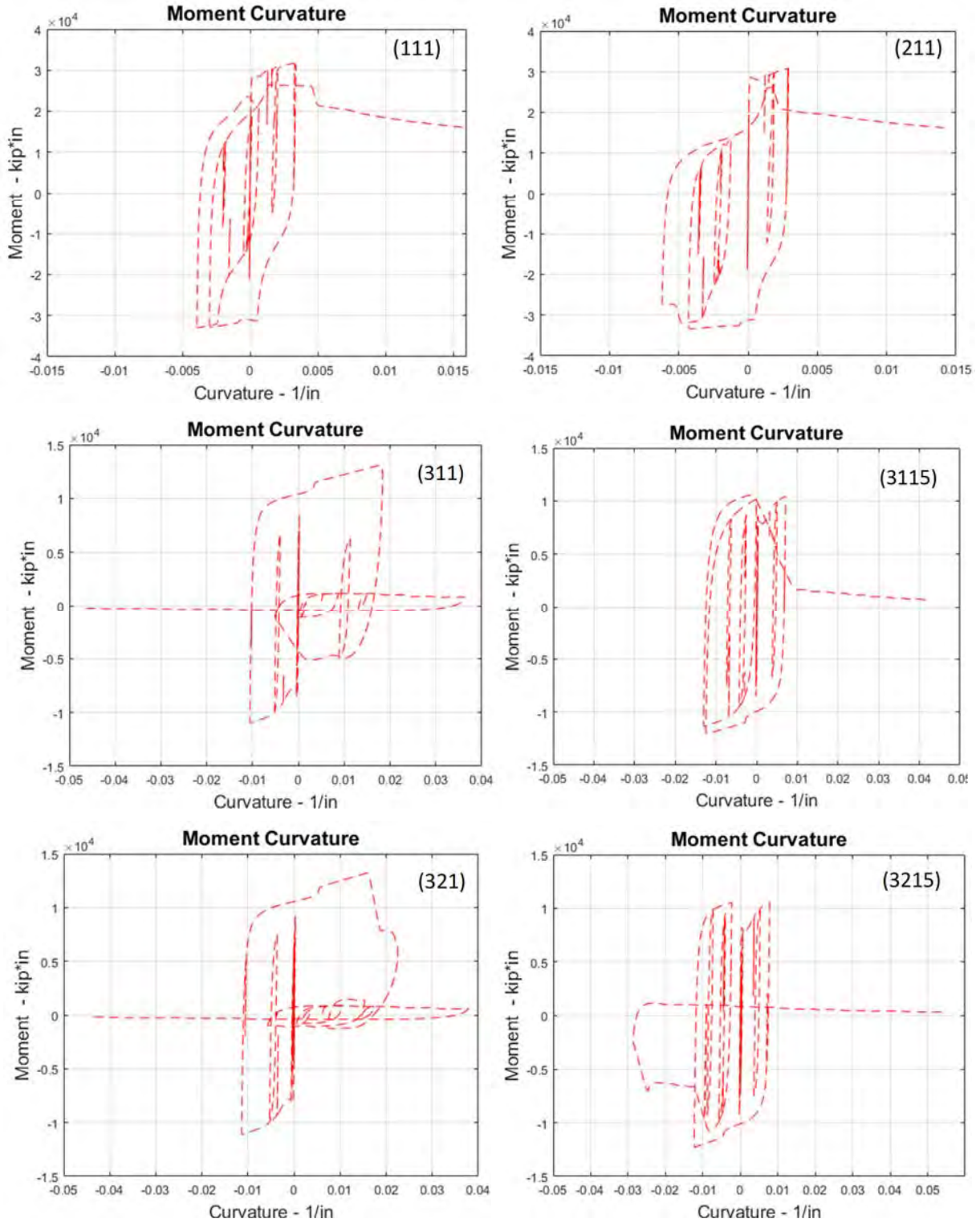
Figure 9-11. Moment Curvature relationship in hinges
