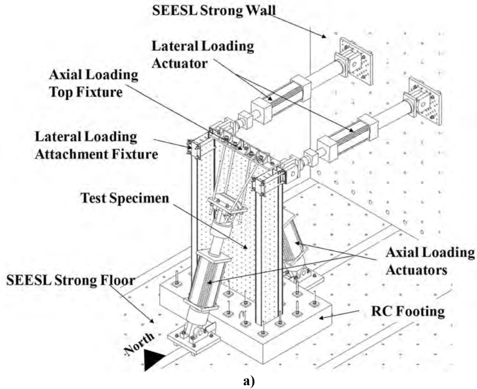
a) Figure 7-64. Details of test setup of the C-shaped wall specimens: a) isometric view; b) West elevation view; c) South elevation view, and; d) top view
