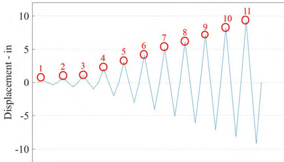
Figure 7-3. Loading Protocol for trial walls
