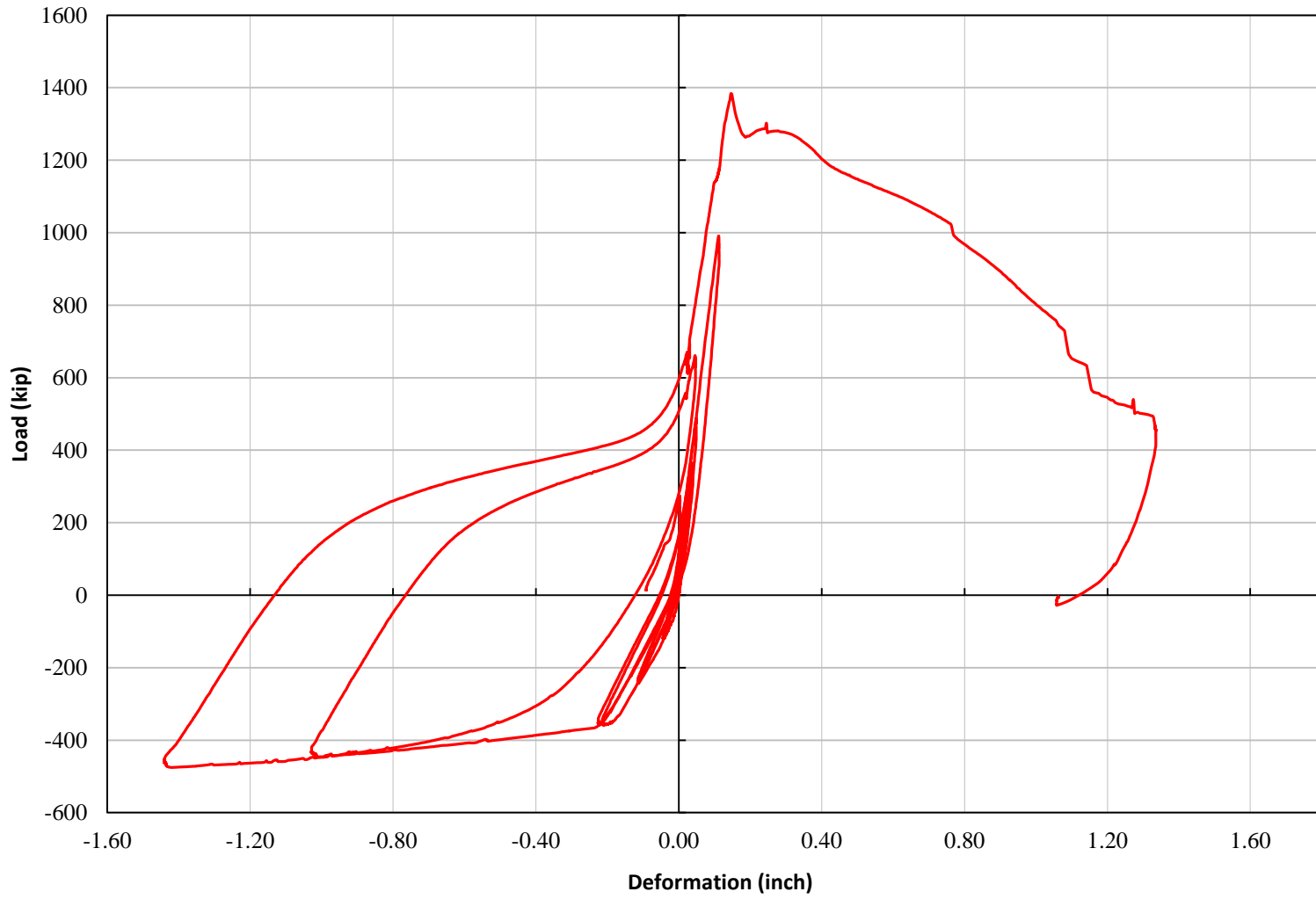
Figure 4-4: Head-travel for TS02
