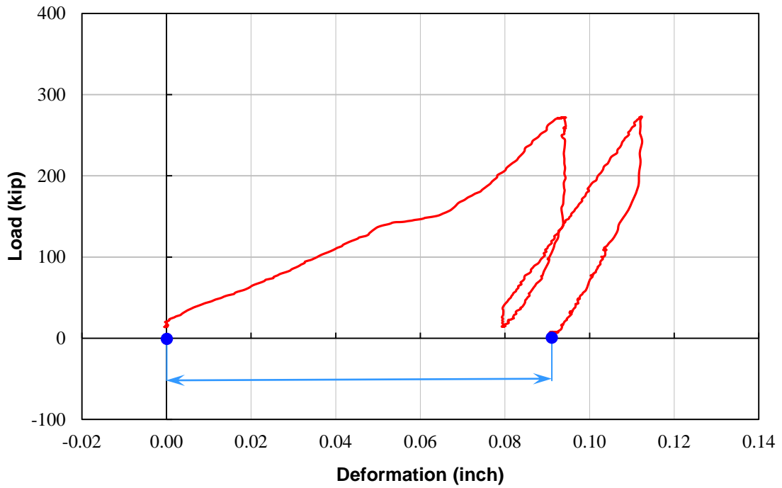
Figure 4-6: Head-travel at the end of Load Step 04 for TS02
