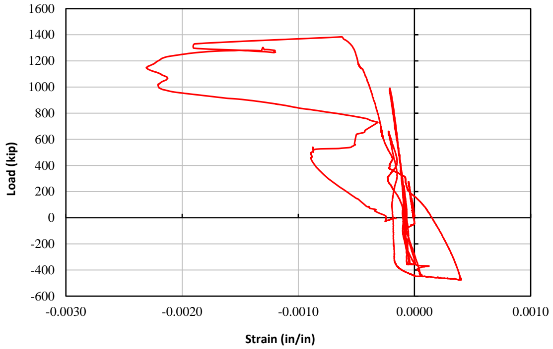
Figure 4-70: Strain gage H2-R3-5 for TS02
