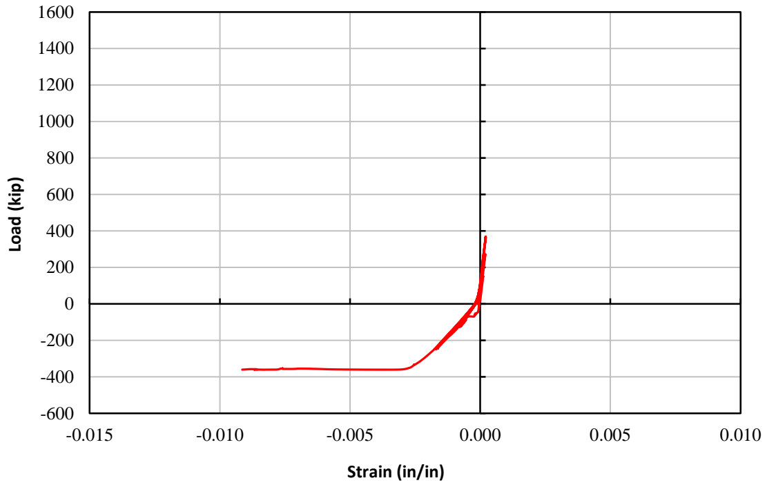
Figure 4-26: Strain gage L1-R7-4 for TS01
