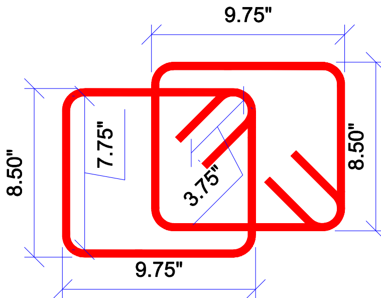
Figure 3-5: Confinement hoop-pair size
