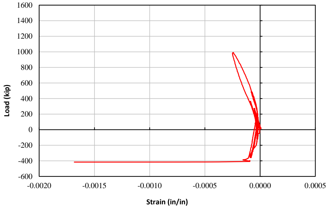
Figure 4-64: Strain gage H1-R3-4 for TS02
