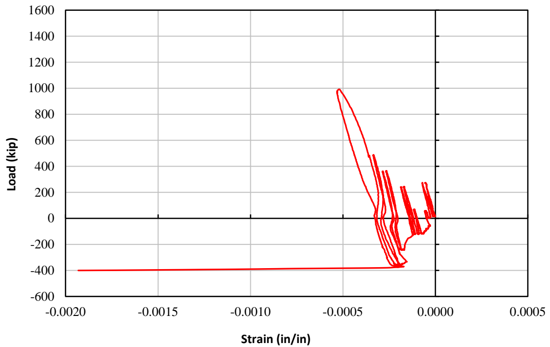
Figure 4-61: Strain gage H1-R3-1 for TS02
