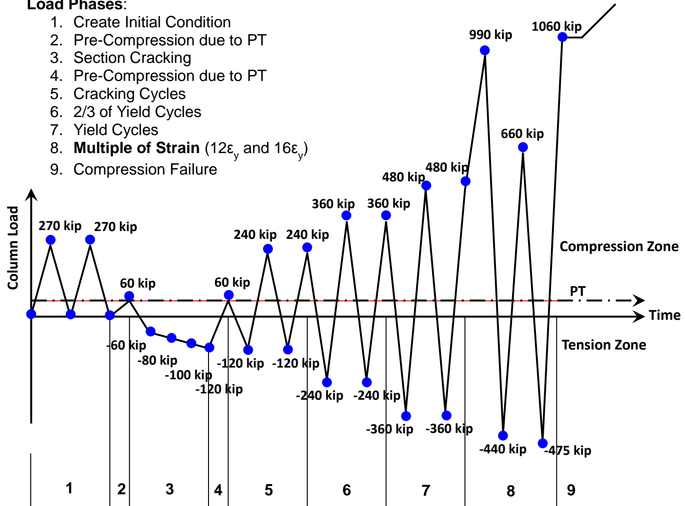
Figure 3-18: Loading protocol for TS02 including load phases notation
