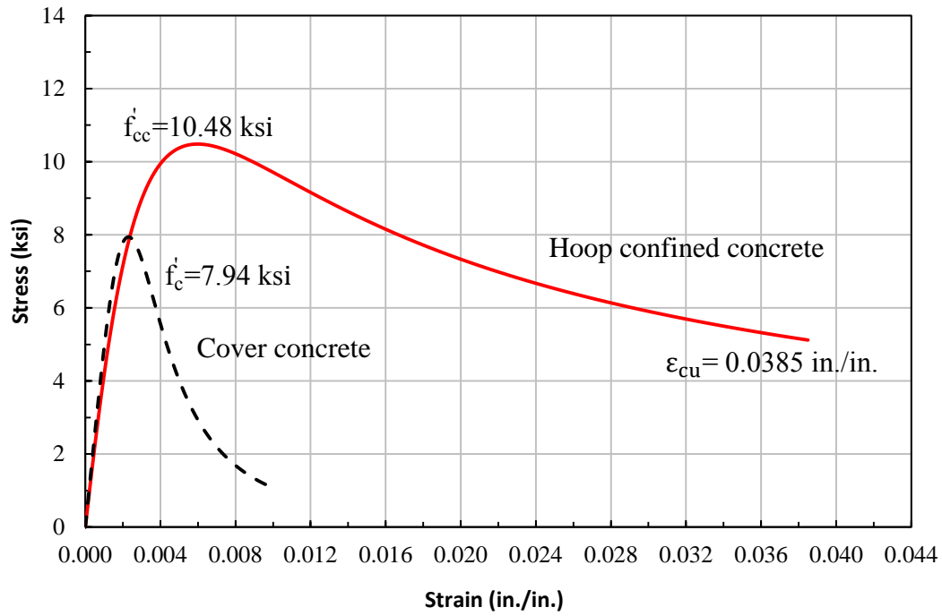
Figure 5-26: Mander (1988) stress-strain model with peak stress and the corresponding strain values from Oh (2002)
