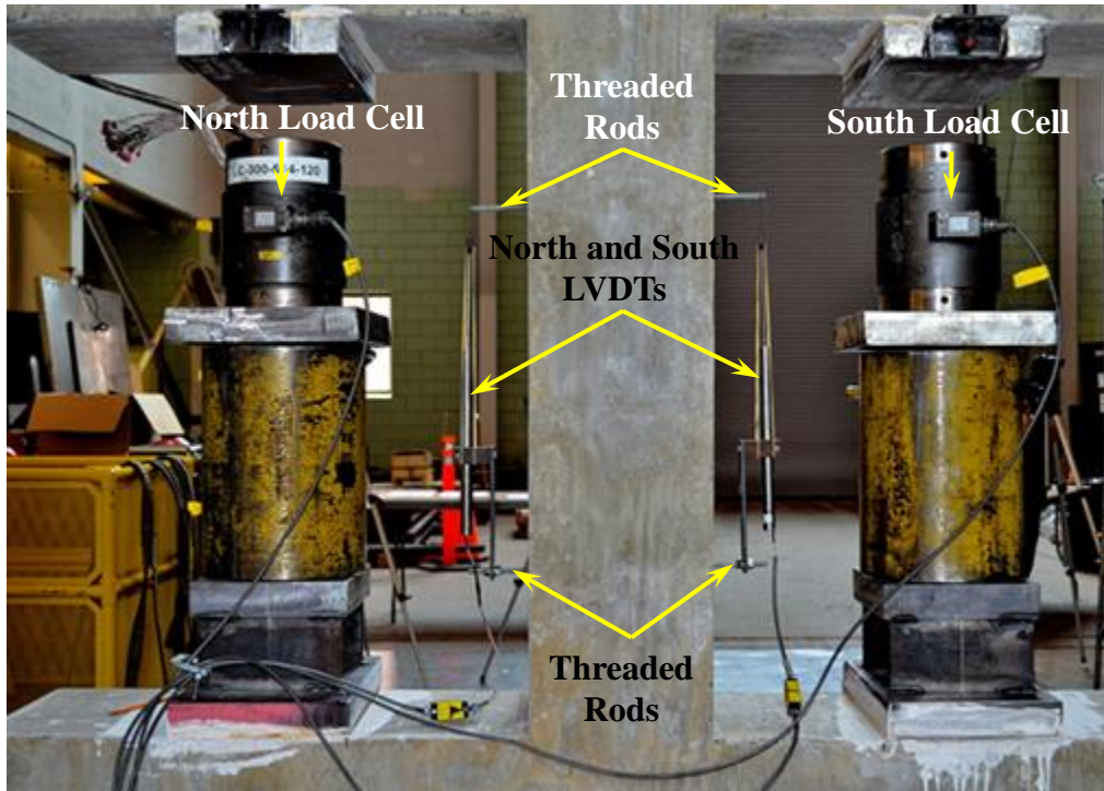
Figure 3-28: Instrumentation before loading
