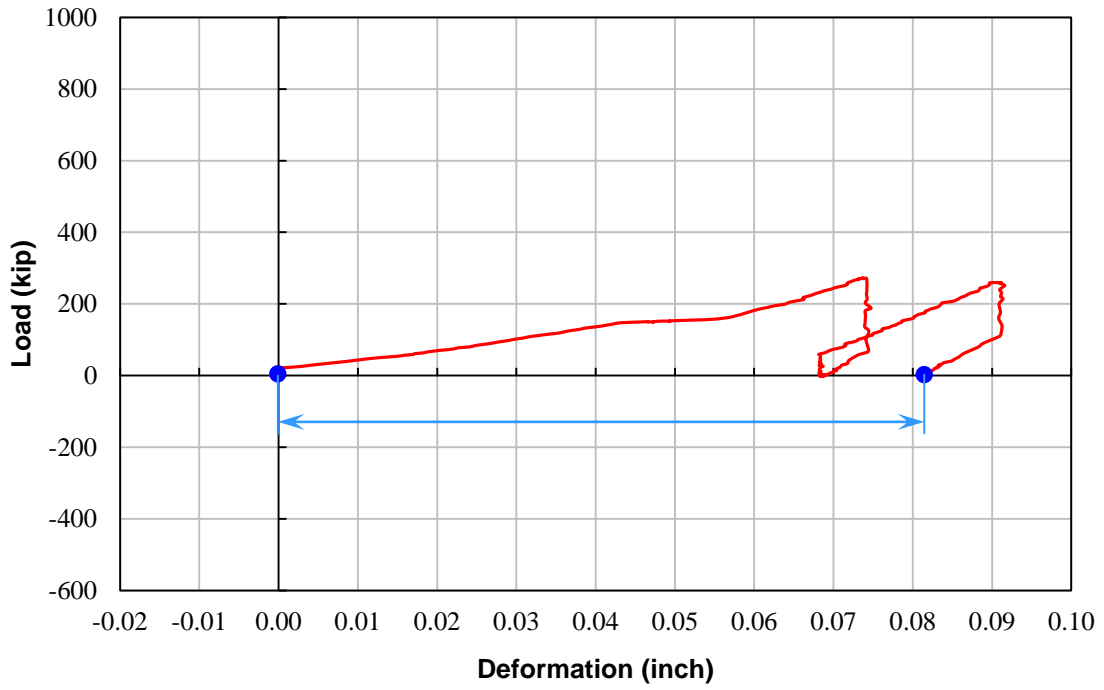
Figure 4-5: Head-travel at the end of Load Step 04 for TS01
