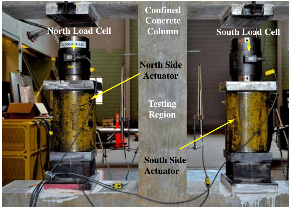
Figure 3-12: Actuator setup before loading
