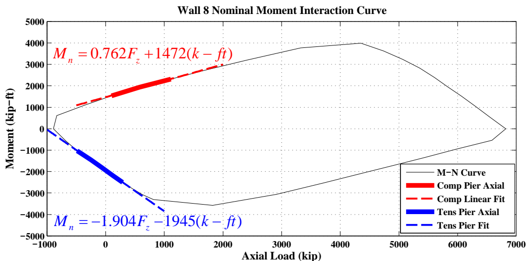
Figure 8.2: Wall 8 M-N Interaction Curve
