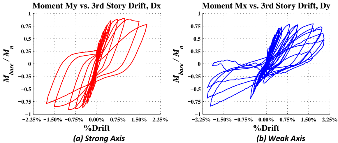
Figure 8.3: Wall 8 normalized moment overall hysteresis
