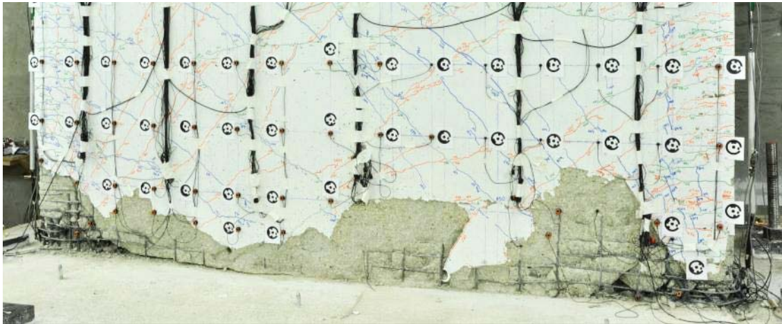
Figure 9.4: Wall 8 web
